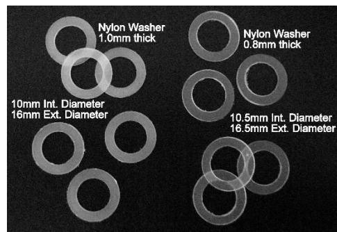
NYLON WASHERS 0.8mm thick – Code: EYE343 1.0mm thick – Code: EYE344
