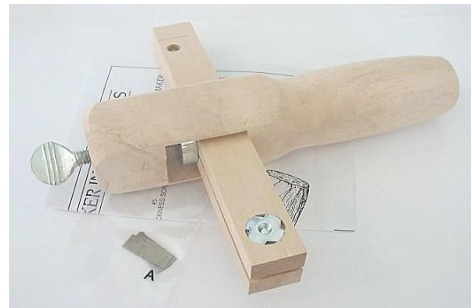
STRAP CUTTER Cuts the softest and heaviest leather Code: TOL220
